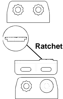
Transducer bracket
